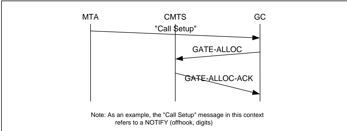
Figure 15 - Sample Signaling of Gate-Alloc
