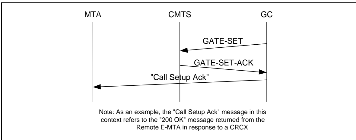
Figure 16 - Sample Signaling of Gate-Set
